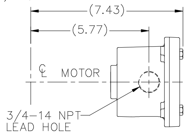
VIEW OF CONDUIT BOX INSTALLED
