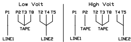
wiring diagram
